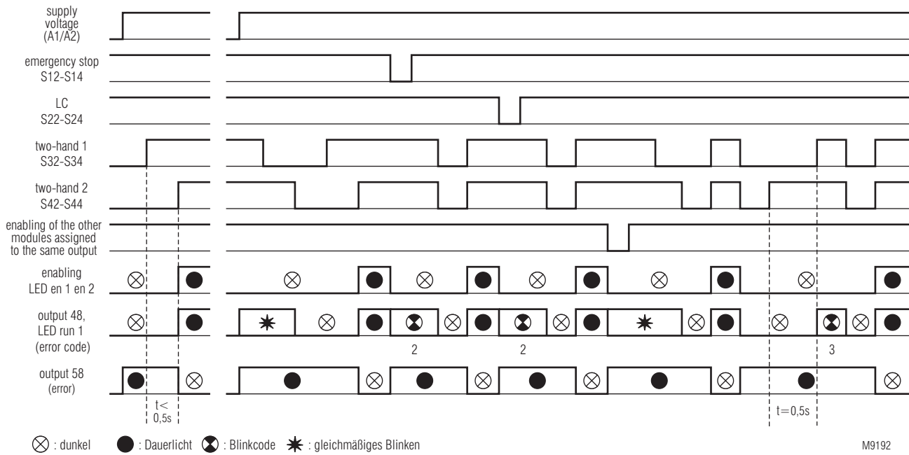
Emergency stop and / or light curtains, manual start, 1 two-hand control type IIC; functions: 6, 7 or 8
